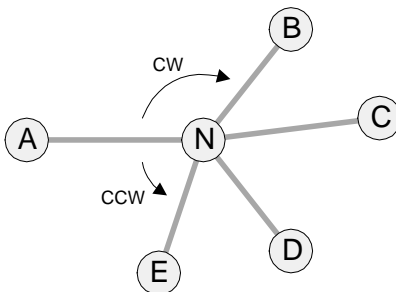
Figure 8: The clockwise and counter-clockwise neighbors of N with respect to A are N 's neighbors that form the smallest clockwise (CW) and counter-clockwise (CCW) angles to A with respect to N . Here, B = CW_A(N) and E = CCW_A(N) . When N sends a neighbor message to A it includes the CW and CCW neighbors.
