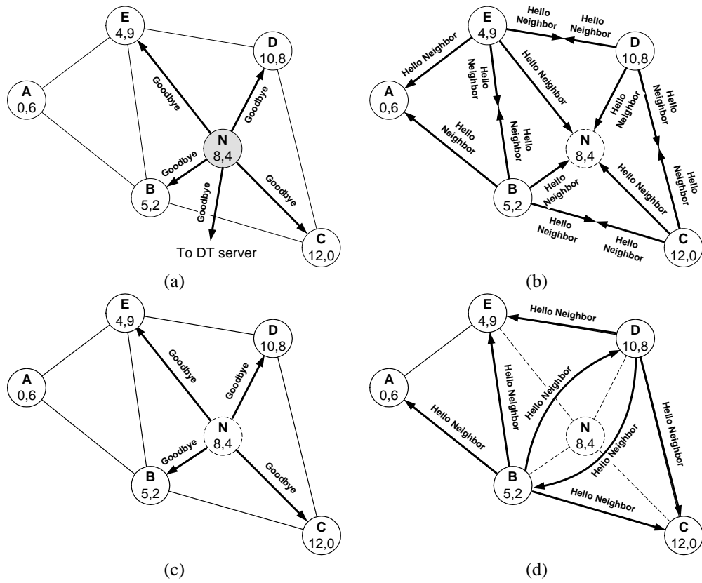
Figure 10: Node N with coordinates coord(N) = (8, 4) leaves the overlay network.
