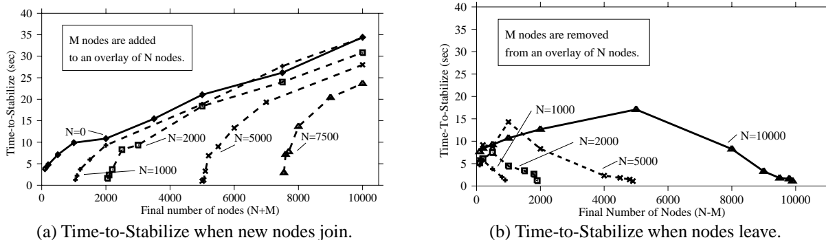
Figure 13: Time-to-Stabilize when nodes join or leave the overlay network. In (a), M new nodes are added to an overlay of N nodes. The time to stabilize is the time until the resulting overlay network of N + M nodes has formed a Delaunay triangulation. In (b), there are N nodes initially, and M nodes depart at the beginning of the experiment. Here, the time to stabilize is the time until the resulting overlay network of N - M nodes has formed a Delaunay triangulation.
