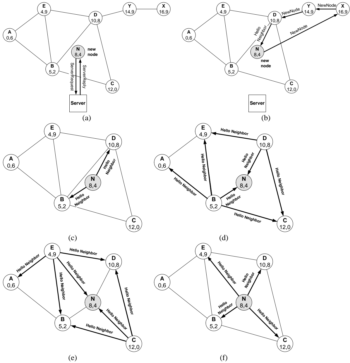
Figure 9: Node N with coordinates coord(N) = (8, 4) joins the overlay network. Note that in (a) and (b), we have omitted some edges from the Delaunay triangulation for the sake of simplicity, and in (c)–(f), we have omitted nodes X and Y .
