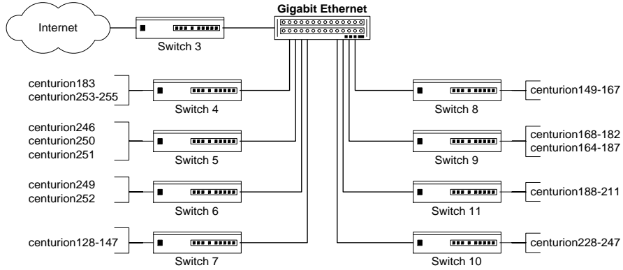
Figure 11: Network topology of the Centurion cluster. The figure only shows equipment involved in the experiments. Switches 3 to 11 are Ethernet Switches with 100 Mbps ports and one 1 Gbps uplink. All links are full-duplex. Hosts are labeled ‘centurion N ’, where N is a number. All hosts have valid IP addresses and may run other applications at the time of the experiments. At most 100 nodes are involved in any single experiment.
