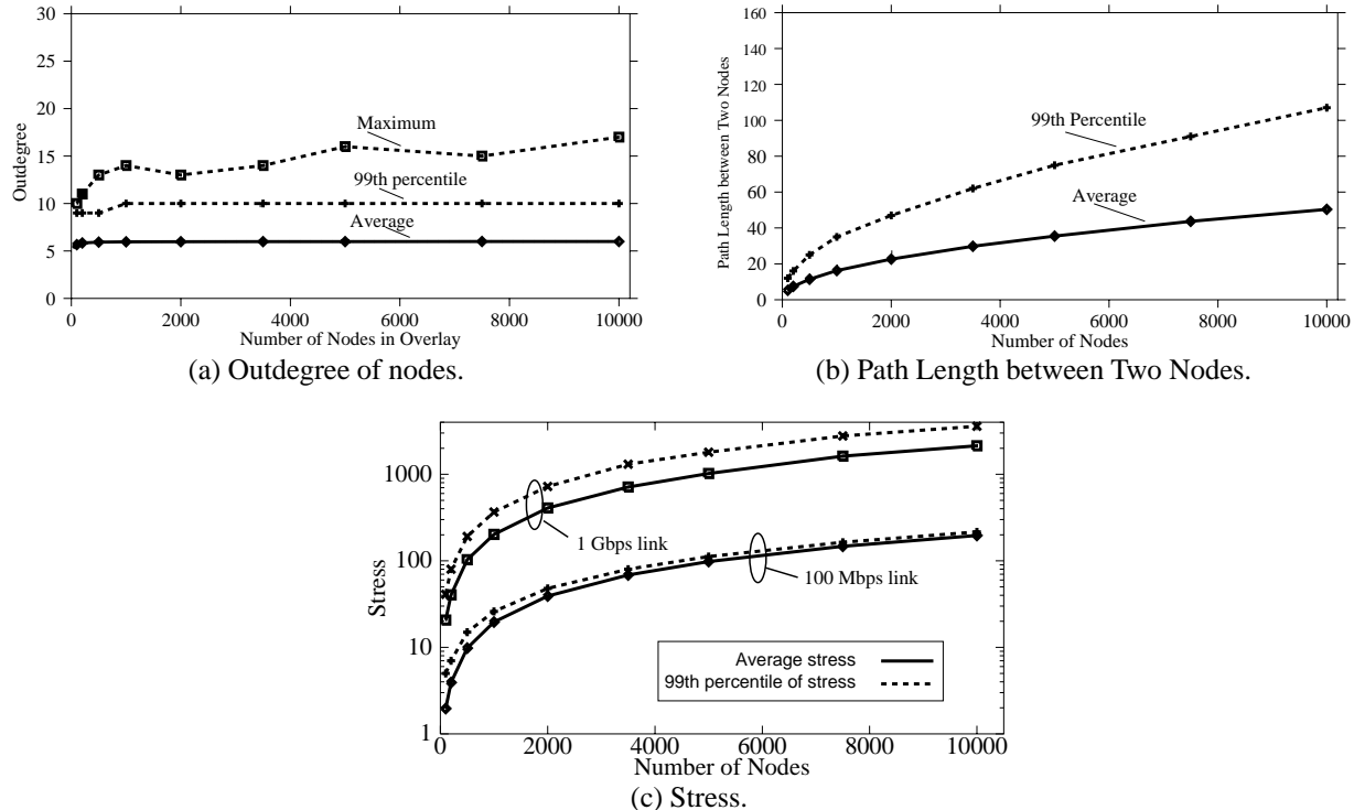
Figure 12: Outdegree of nodes, path length between two nodes, and stress of links in the overlay network. Each data point shows the results from five generated graphs. In (b), the values for the path length are computed from 1 000 randomly selected node pairs. In (c), the values for the ‘stress’ of a link are computed for at most 1000 randomly selected multicast trees.
