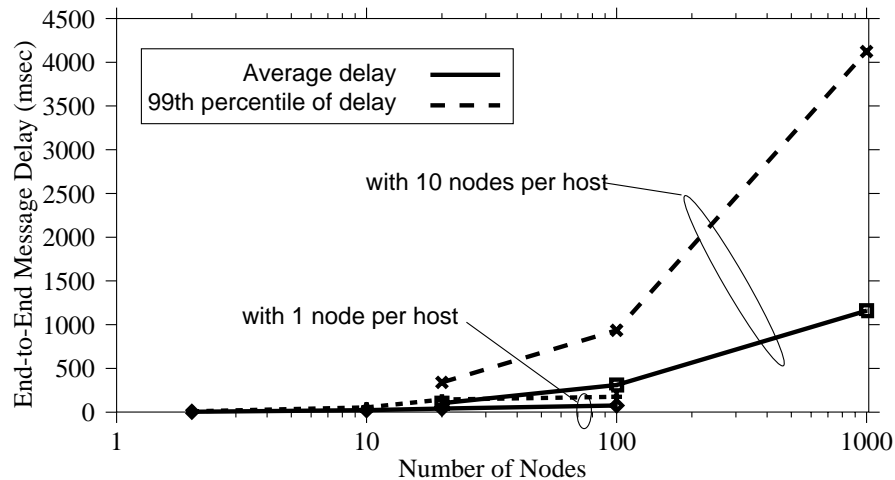
Figure 17: Measured end-to-end delay of messages. The plots show average delays and 99th percentile of delays for receivers in a set of multicast trees. We present two measurements: (1) 100 MB bulk data transfers for an overlay with N = 2 - 100 nodes, where at most one node is assigned to each host; and (2) 10 MB bulk data transfer for an overlay with N = 20 - 1000 nodes, where always 10 nodes are assigned to each host.
