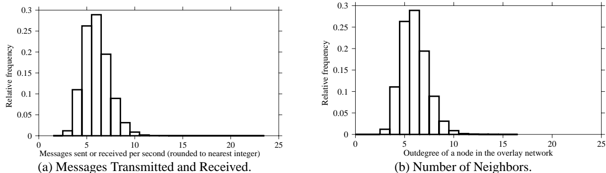
Figure 15: Distribution of the number of messages (sent and received) of a node and the number of neighbors per node in an overlay network with 10 000 nodes. The histogram in (a) shows the average number of messages sent and received by a node in a 1-second time interval.
