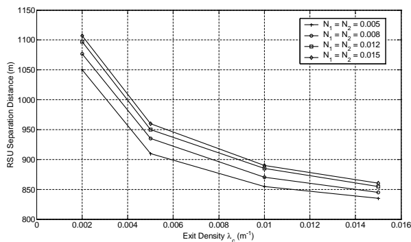
Fig. 6. The maximal RSU separation distance with different road junction and vehicle densities.
