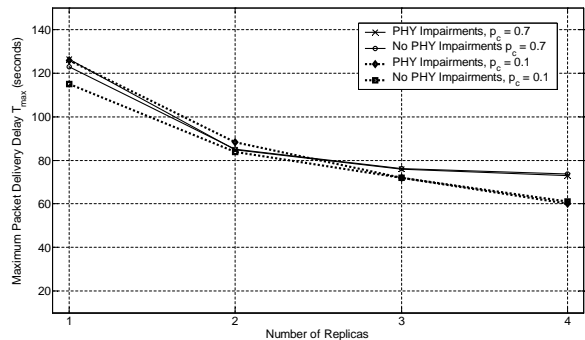
Fig. 9. Maximum packet delivery delay ( T_{max} ) versus the number of replicas with the existence of physical layer impairments.
