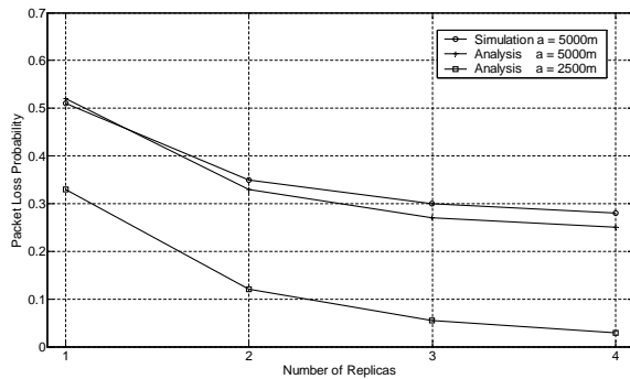
Fig. 10. Packet loss probability versus the number of replicas.
