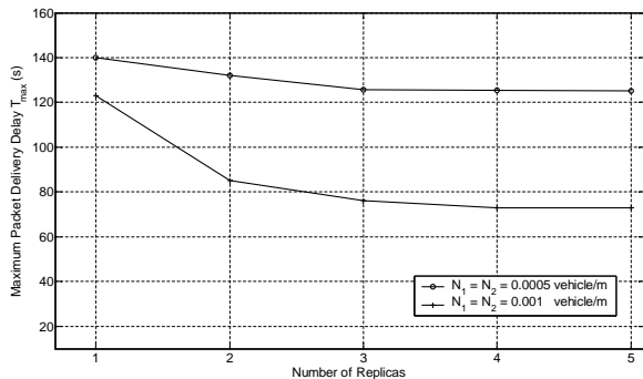
Fig. 8. Effect of vehicle density on the number of replicas required to reduce packet delay.
