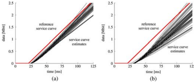
Fig. 9. Experiment 2: Rate scanning with different cross traffic. (a) Exponential cross traffic. (b) Pareto cross traffic.
