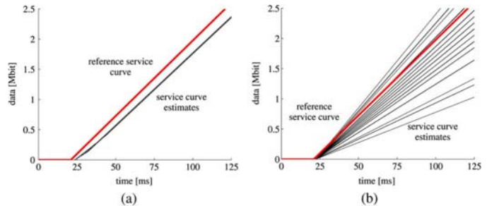
Fig. 8. Experiment 1: Service curve estimates with CBR cross traffic (Each of the graphs shows the reference service curve and the results of 100 repeated estimates of the service curve). (a) Rate Scanning. (b) Rate Chirp.
