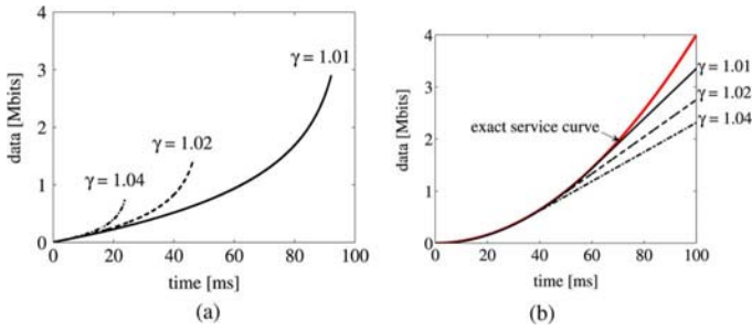
Fig. 5. Service curve estimation with rate chirps. (a) Rate chirps. (b) Rate chirp results with different spread factors.
