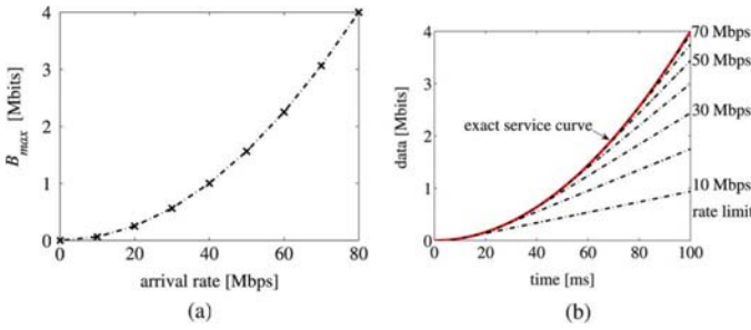
Fig. 4. Service curve estimation with rate scanning. (a) Maximum backlog B_{\max}(r) . (b) Rate scanning results with different rate limits.
