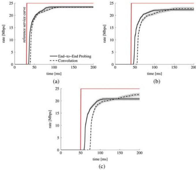
Fig. 12. Experiment 4: Derivative of service curves in multinode measurements. (a) Two bottleneck links. (b) Three bottleneck links. (c) Four bottleneck links.
