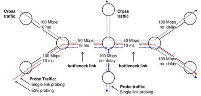
Fig. 11. Topology with multiple bottleneck links.
