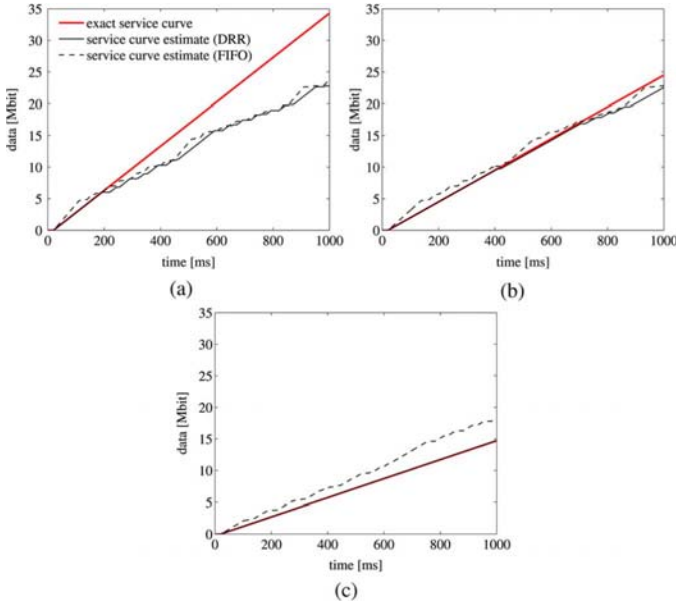
Fig. 3. Example: Passive measurement simulation with a video source. (a) C = 70 Mbps. (b) C = 50 Mbps. (c) C = 30 Mbps.
