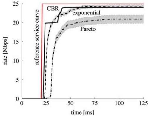
Fig. 10. Results from Experiments 1–2: Derivative of service curves.
