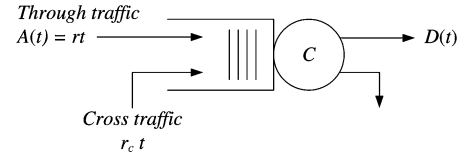
Fig. 6. FIFO system with probe and cross traffic.
