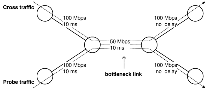
Fig. 7. Dumbbell topology.
