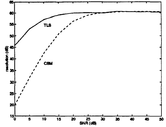
Fig. 1 The resolution of the TLS and CSM methods for a scenario with two closely separated sources at 10 and 14 degrees.
