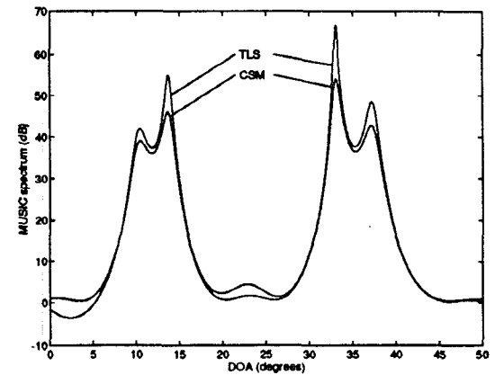
Fig. 3 The MUSIC spectrum for a scenario with 4 equi-power wideband sources at 10, 14, 33, and 37 degrees arriving at a uniform linear array of 20 sensors.
