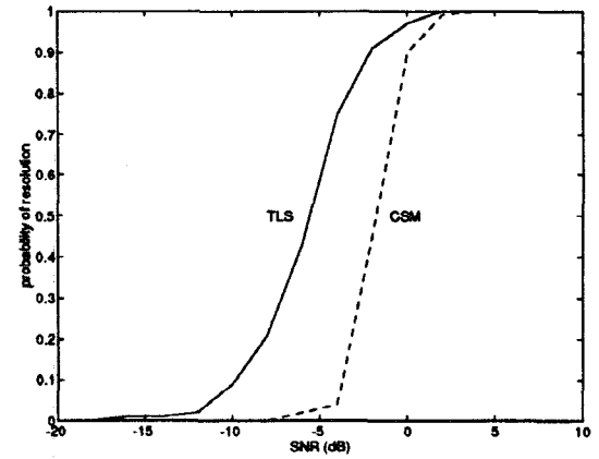
Fig. 2 The probability of resolution for the TLS and CSM methods for a scenario with two closely separated sources at 10 and 14 degrees.
