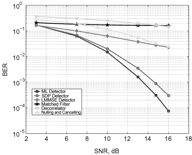
Fig. 2. BER as a function of SNR for different detectors. Simulation parameters: BPSK modulation n = 10 .
