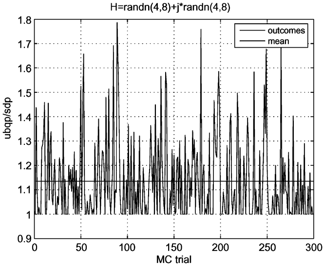
Fig. 3. Upper bound on v_{ap}/v_{sdp} for m = 8 , n = 4 , over 300 realizations of complex Gaussian i.i.d. channel vector entries.
