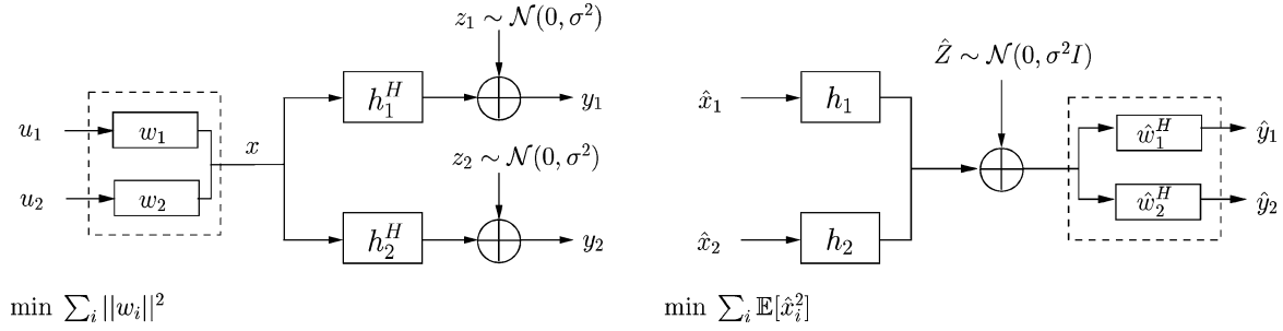
Fig. 1. Uplink-downlink beamforming duality can be interpreted as a Lagrangian duality in convex optimization.
