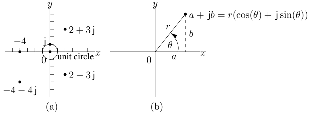
Figure 1: (a) Several points in the complex plane. (b) The polar form of a complex number.
