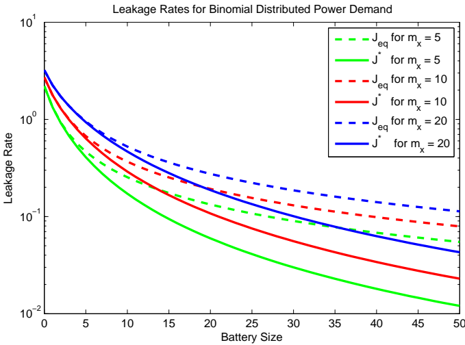
Fig. 3: A comparison of the performance of q_{eq} \in \mathcal{Q}_B as defined in (18) with the optimal leakage rate for i.i.d. Binomial distributed demand \text{Binomial}(m_x, 0.5) for m_x = \{5, 10, 20\} .
