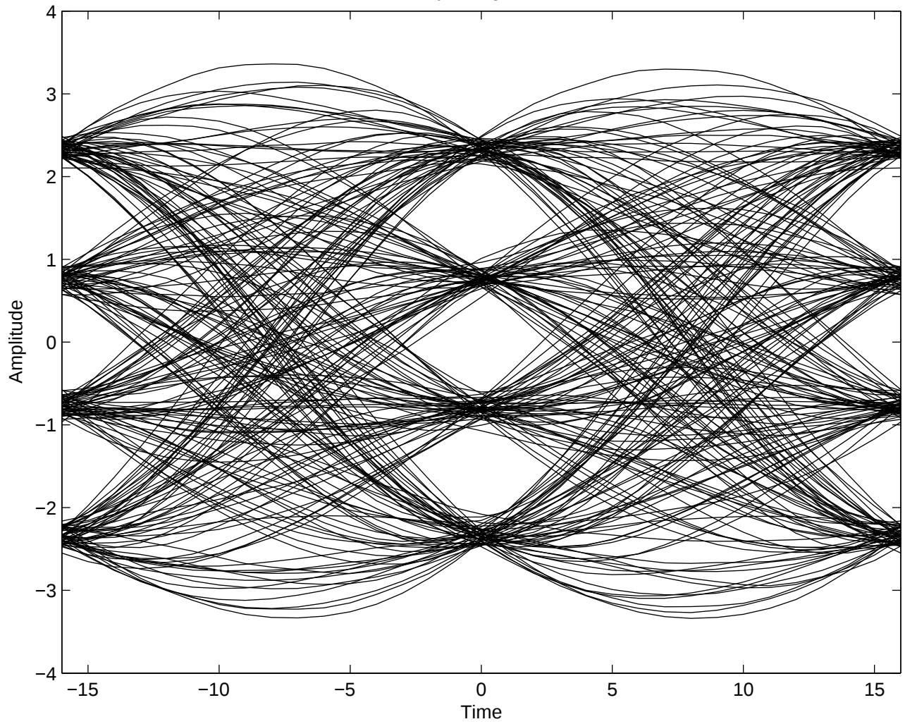
Eye Diagram
