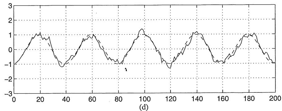
Figure 7.9 Noise cancellation example. (a) Noise corrupted sinusoid, (b) Reference signal used by secondary sensor, (c) Output of sixth-order Wiener noise canceller, (d) Output of twelfth-order Wiener noise canceller.
