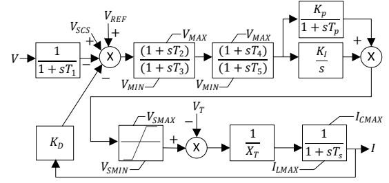
Figure 3. STATCOM control system block diagram
