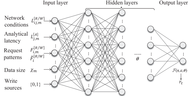
Fig. 5. NN structure for data placement.
