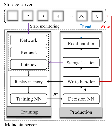
Fig. 6. Production and training system of DataBot+.
