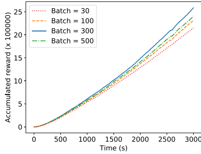
Fig. 14. Impact of batch size |\mathcal{B}| .
