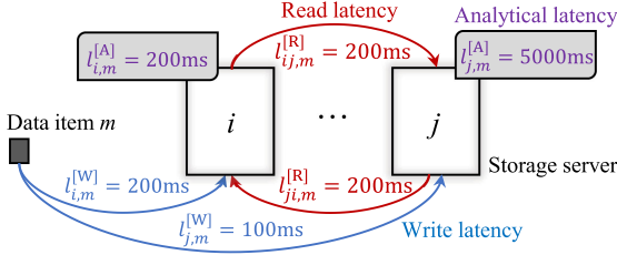
Fig. 4. An example of the storage location selection between server i and j for data item m when the data read/write and analytical latencies are considered.
