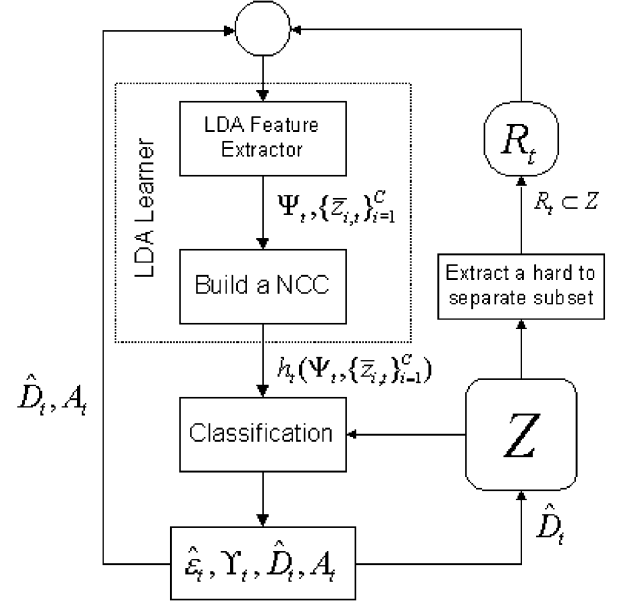
Fig. 2. Flow chart of the cross-validation mechanism embedded in the proposed boosting framework to weaken the LDA-style learner. The flow chart is based on one iteration, and the NCC denotes the nearest center classifier.
