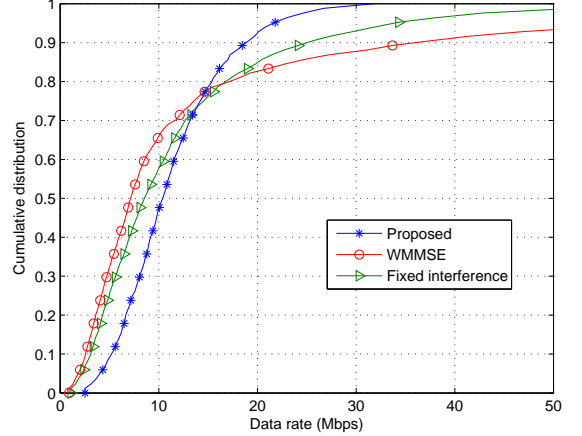
Fig. 1: User-throughput CDF of the different methods
