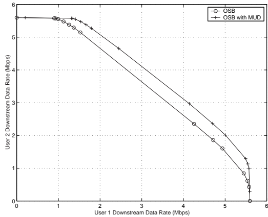
Fig. 2. Achievable rate region for 2-user ADSL downstream using OSB and the joint multiuser detection algorithm
