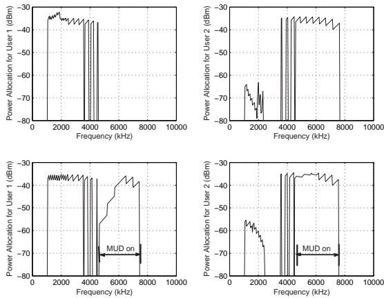
Fig. 3. Power allocations for 2-user ADSL downstream with optimal spectrum balancing alone (top left and right) and with the joint multiuser detection algorithm (bottom left and right)
